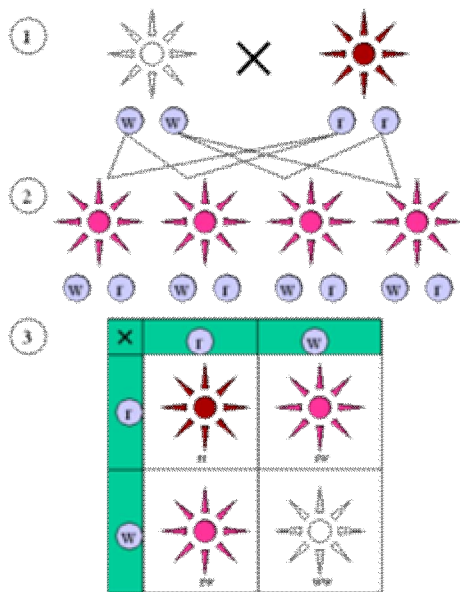
Figure 1: The color alleles of Mirabilis jalapa are not dominant or recessive. (1) Parental generation. (2) F 1 generation. (3) F 2 generation. The "red" and "white" allele together make a "pink" phenotype, resulting in a 1:2:1 ratio of red:pink:white in the F 2 generation.
