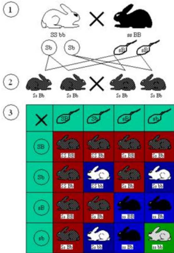
Figure 3 : Two traits (black/white and short/long hair, with black and short dominant) show a 9:3:3:1 ratio in the F 2 generation. (S=short, s=long, B=black, b=white hair) (1) Parental generation. (2) F 1 generation. (3) F 2 generation. Results : 9x short black hair, 3x long black hair, 3x short white hair, 1x long white hair.
