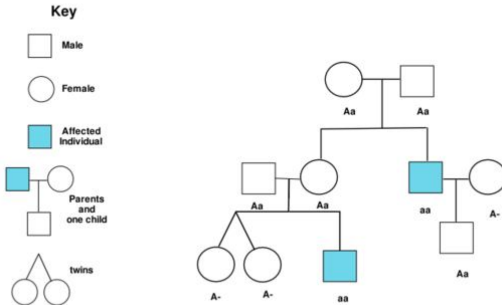
Figure 4. A pedigree chart following a recessive trait.
