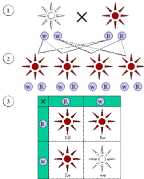
Figure2 : Dominant and recessive phenotypes. (1) Parental generation. (2) F 1 generation. (3) F 2 generation. Dominant (red) and recessive (white) phenotype look alike in the F 1 (first) generation and show a 3:1 ratio in the F 2 (second) generation
