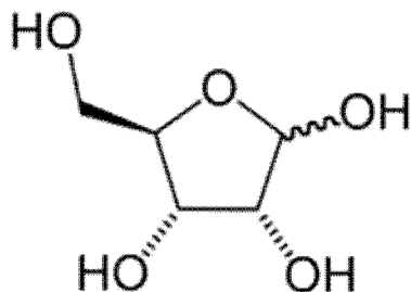
A conventional skeletal formula
