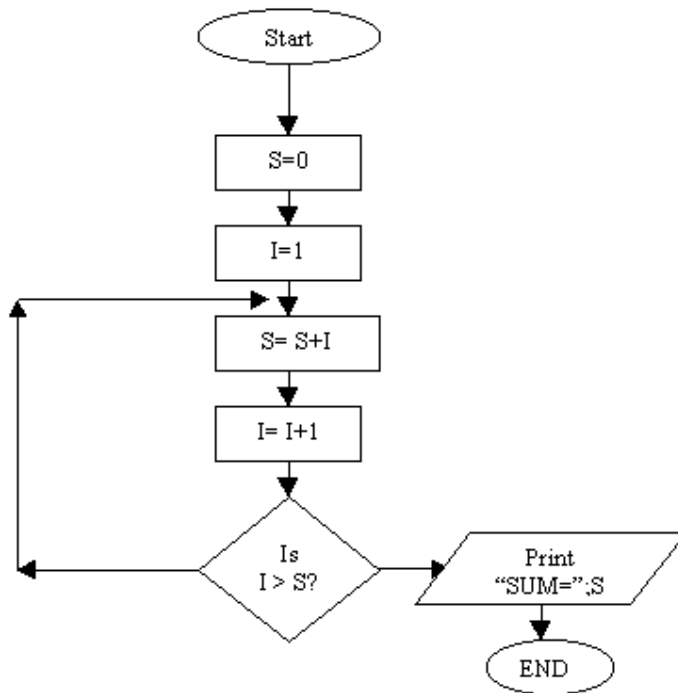
Fig 5.3 Program Flowchart
