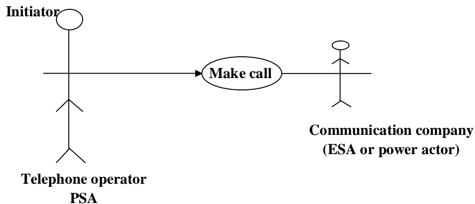
Fig. 4.2: Bi-directional Association
