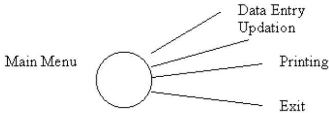
Figure 5.6: Decision Tree
