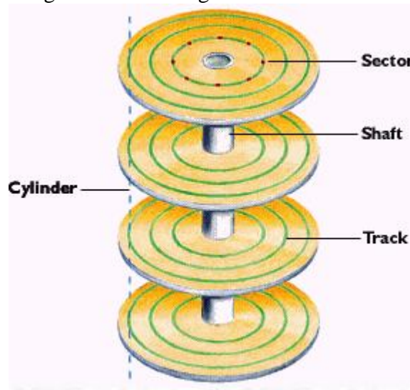
Fig. 8: Disk Cylinder
